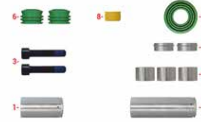
KISA PERNO 37,70x76 UZUN PERNO 38x63/118 MAXX22 T - SCHMITZ DORSE
